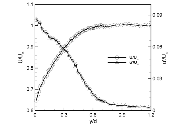
Fig. 3 Approach boundary-layer profiles measured at x/d = -2.95 and z = 0 . U_\infty = 29 \text{ ft/s} .
