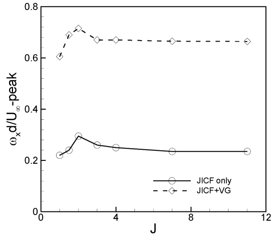
Fig. 12 Variation of flowfield properties with J measured at x/d = 10 : a) location of peak mean velocity at z = 0 (jet penetration), b) peak turbulence intensity, and c) peak streamwise vorticity (solid curves: JICF only case; dashed curves: JICF-plus-VG case).
