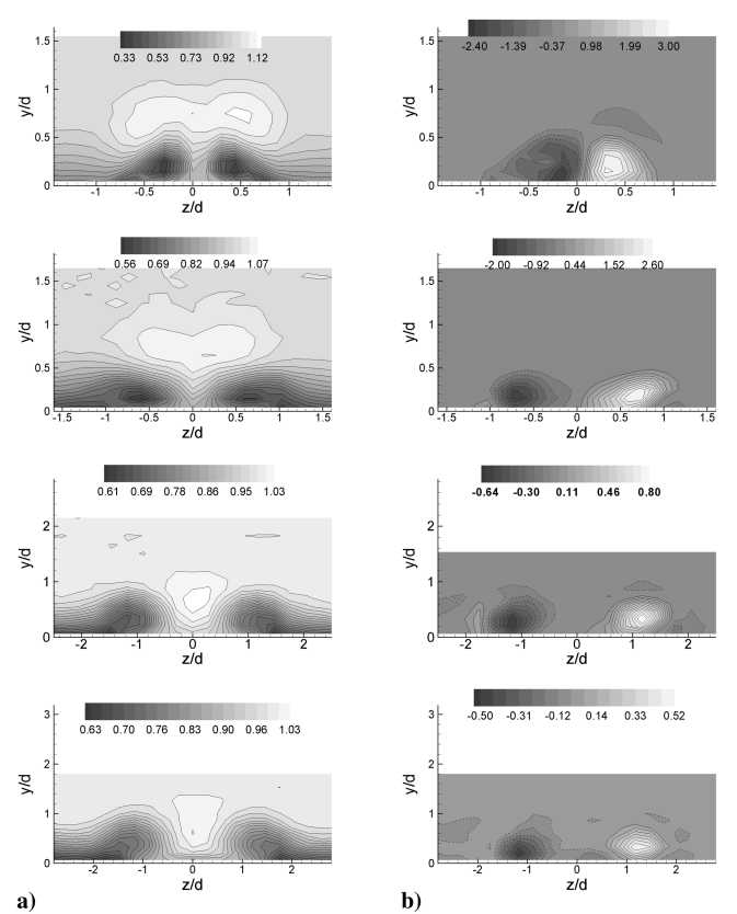
Fig. 7 Flowfield properties for VG-plus-JICF case. In each figure, from top to bottom, the data are for surveys at x/d = 3.1, 5, 10, and 15 . a) Mean velocity ( U/U_\infty ), and b) streamwise vorticity ( \omega_x d/U_\infty ).
