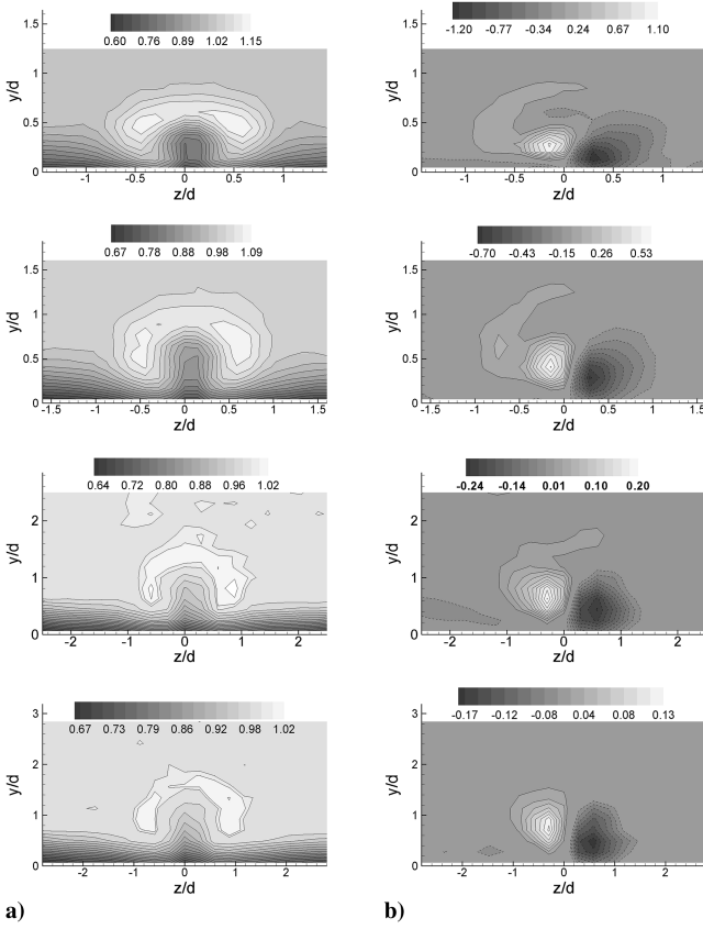
Fig. 5 Flowfield properties for JICF-only case. In each figure, from top to bottom, the data are for surveys at x/d = 3.1, 5, 10, and 15 . a) Mean velocity ( U/U_\infty ), and b) streamwise vorticity ( \omega_x d/U_\infty ).
